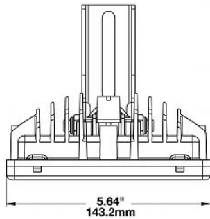
Dimensions in inches (mm in parentheses). Dimensions are for reference only.
