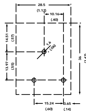
Punching diagram for PCB (component side)
