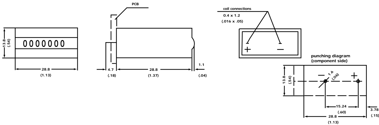
Punching diagram for PCB (component side)
